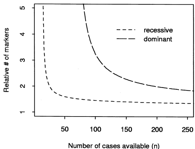
Figure 5 Number of diallelic markers required for a genome screen (80% power and \alpha = .001 ), relative to number of multiallelic markers required, as a function of available sample size. In the recessive disease case the multiallelic marker has six alleles, whereas in the dominant disease case it has eight alleles.
